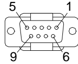
Figure 8-3 Serial Port Pin Assignments
