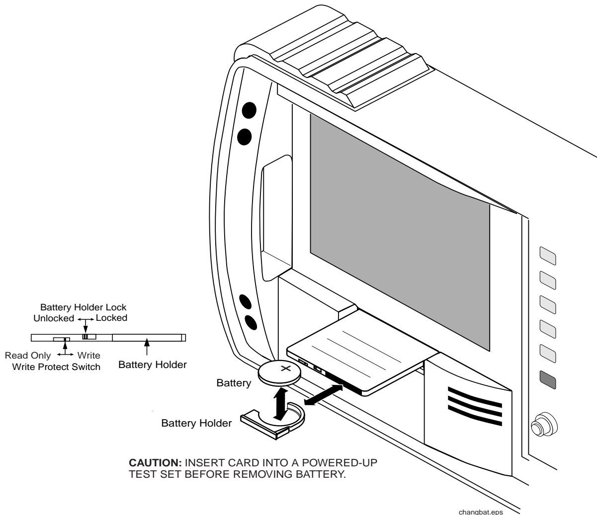
Figure 7-3 Inserting the Battery and Setting the Write-Protect Switch
